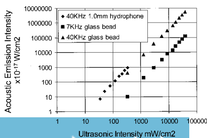
FIG. 3. Acoustic-emission field intensity vs. the combined ultrasonic intensity.
