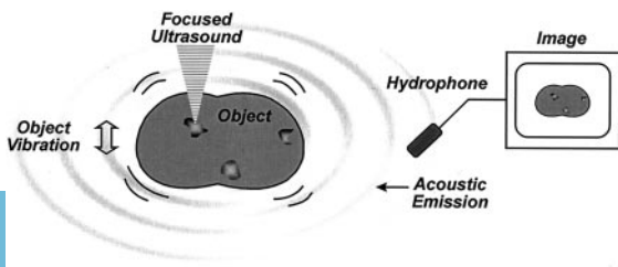
FIG. 1. Principle of ultrasound-stimulated vibro-acoustography.
